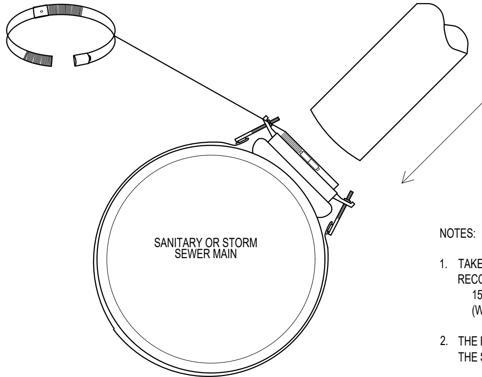
STYLE "CB" SEWER SADDLE
